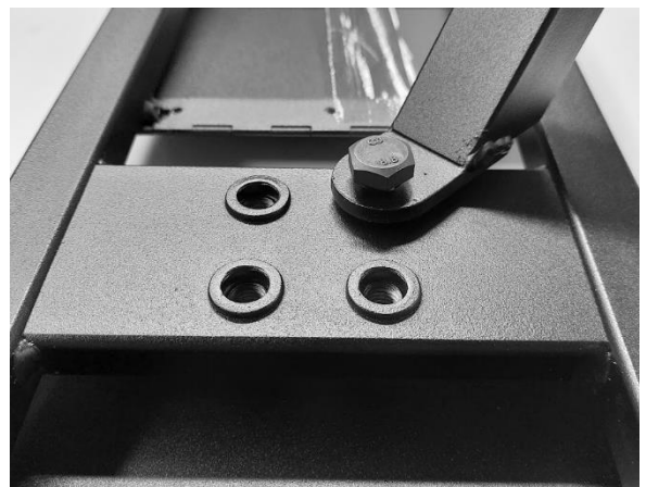
screws M10x20
