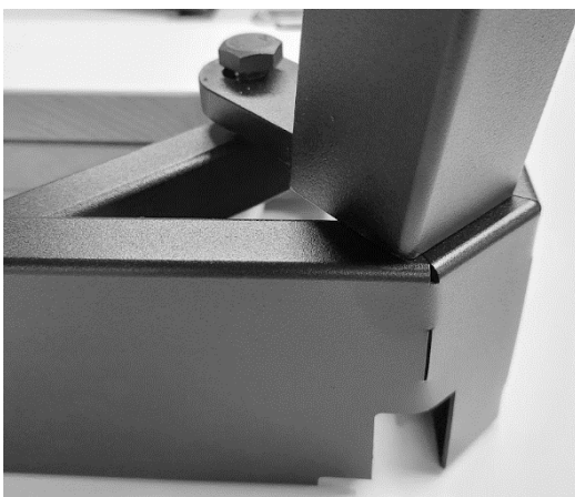
screws M10x30
